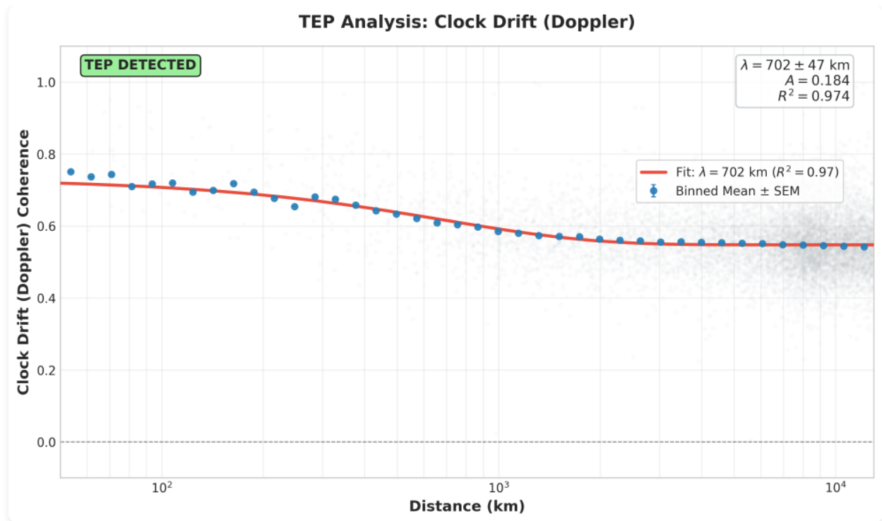
Figure 3.3: Phase coherence of clock drift (derivative of clock bias). The persistence of spatial structure in the derivative is less consistent with a simple random walk artifact.
