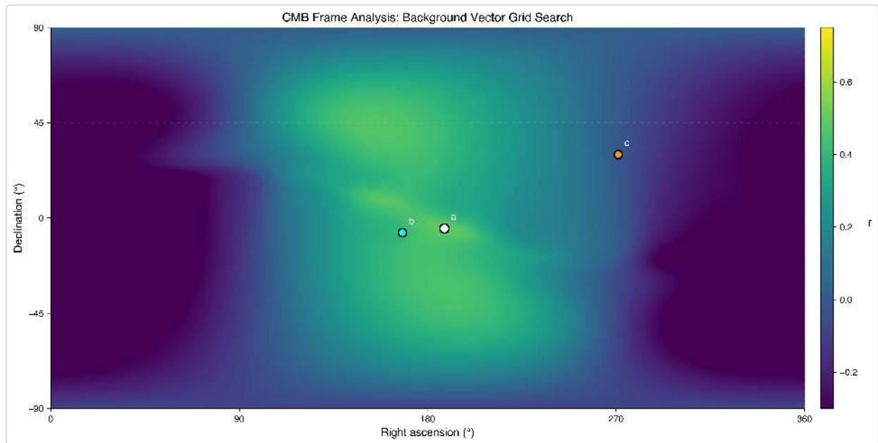
Figure 3.7. Full-sky correlation map for ALL_STATIONS / Multi-GNSS / pos_jitter / phase_alignment. The best-fit direction is RA = 188^\circ , Dec = -5^\circ , corresponding to an angular separation of 20.0^\circ from the CMB dipole. The CMB dipole and Solar Apex reference directions are marked.
