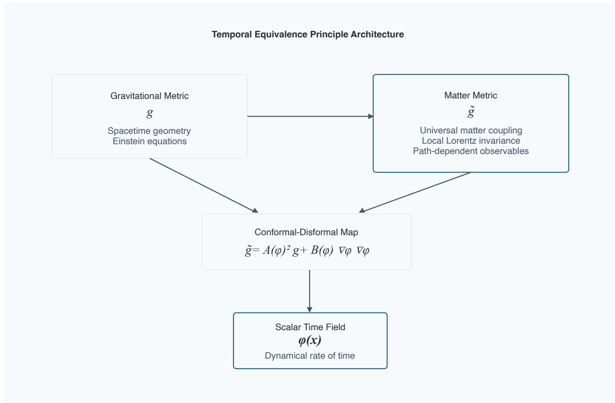
Figure 1. Temporal Equivalence Principle (TEP) architecture. Matter couples to \tilde{g}_{\mu\nu} via a conformal–disformal map controlled by the scalar time field \phi , preserving local Lorentz invariance while enabling new global invariants.
