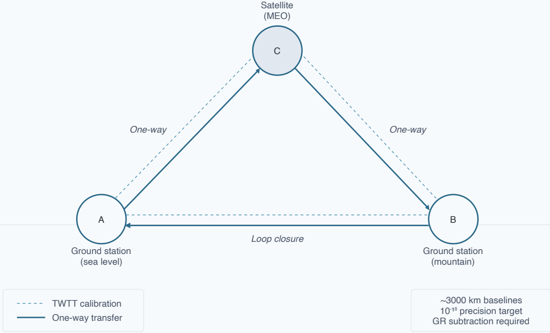
Figure 3. Triangle synchronization experiment geometry. Two ground stations (sea level and mountain) and a medium-Earth-orbit satellite form \sim 3000 km baselines; two-way time transfer calibrates each edge while one-way transfers around the loop probe H_{\text{resid}} after GR subtraction.
